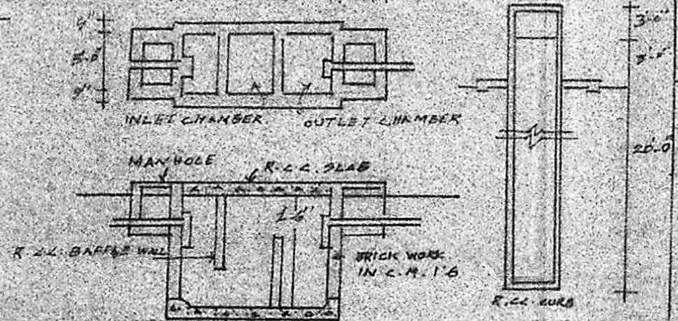
DETAILS OF SEPTIC TANK & 4 DIA WELL
